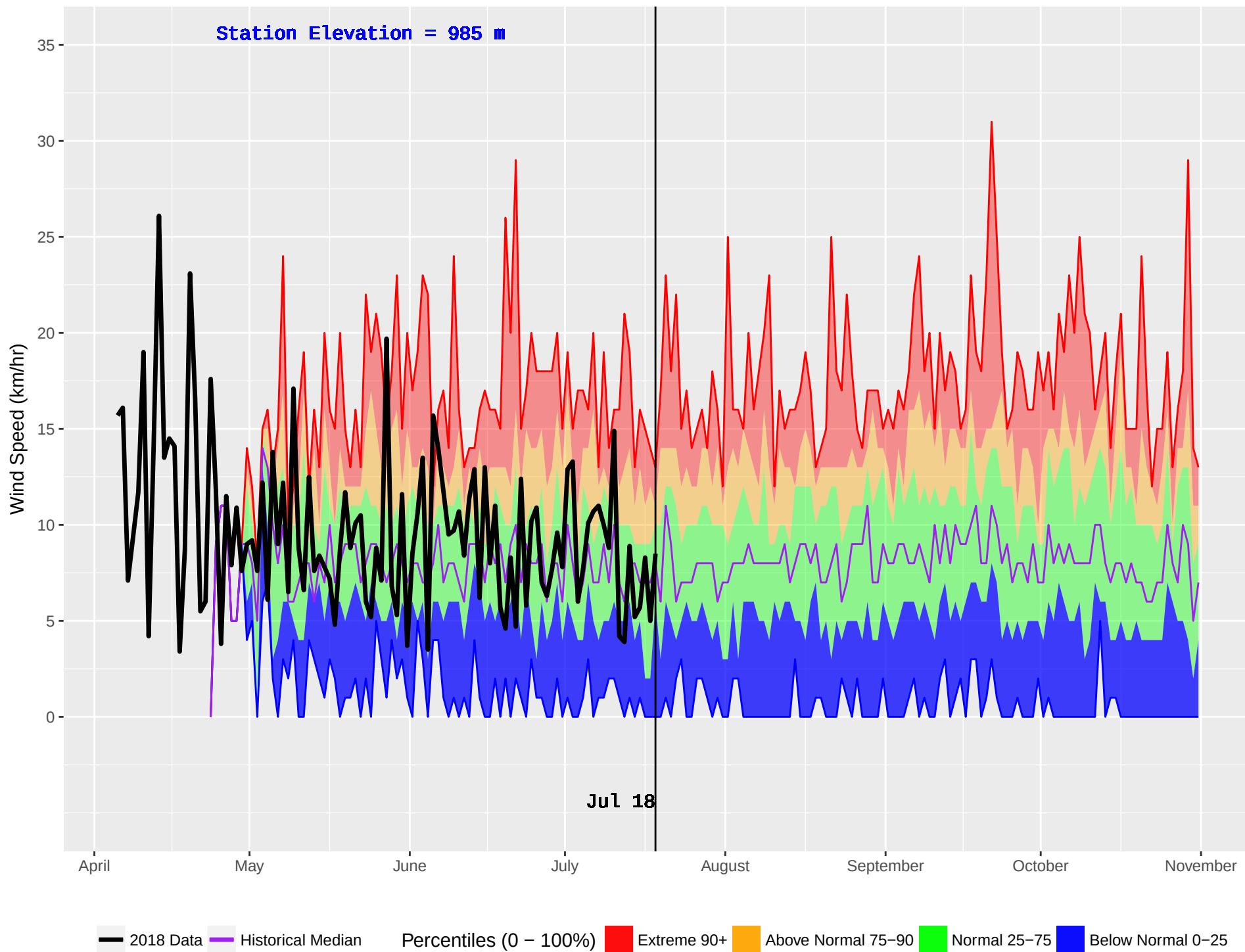
SIFTON (152) : Historical (1988–2016) and Current (2018) Daily Wind Speed
