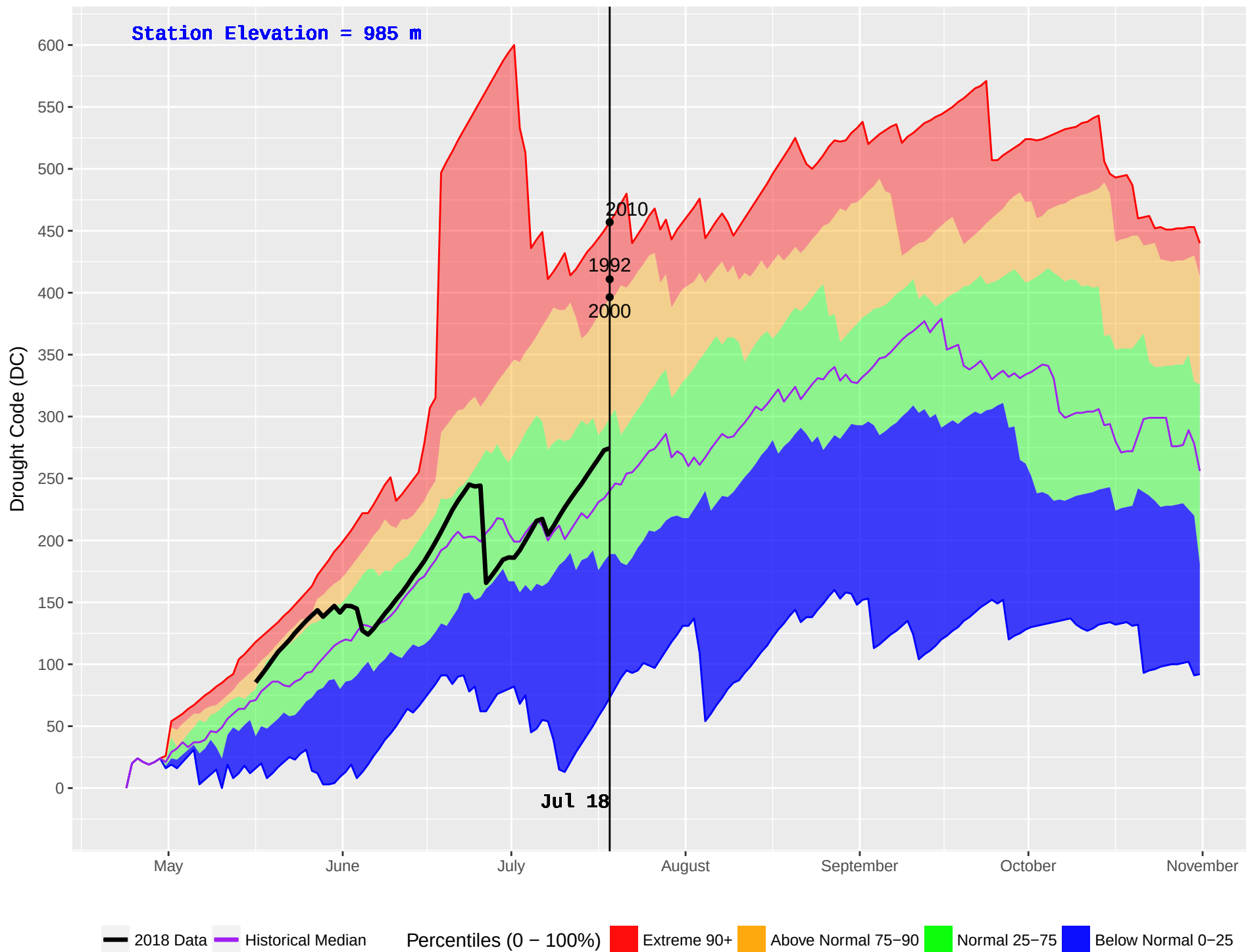
SIFTON (152) : Historical (1988–2016) and Current (2018) Daily Drought Code (DC)
