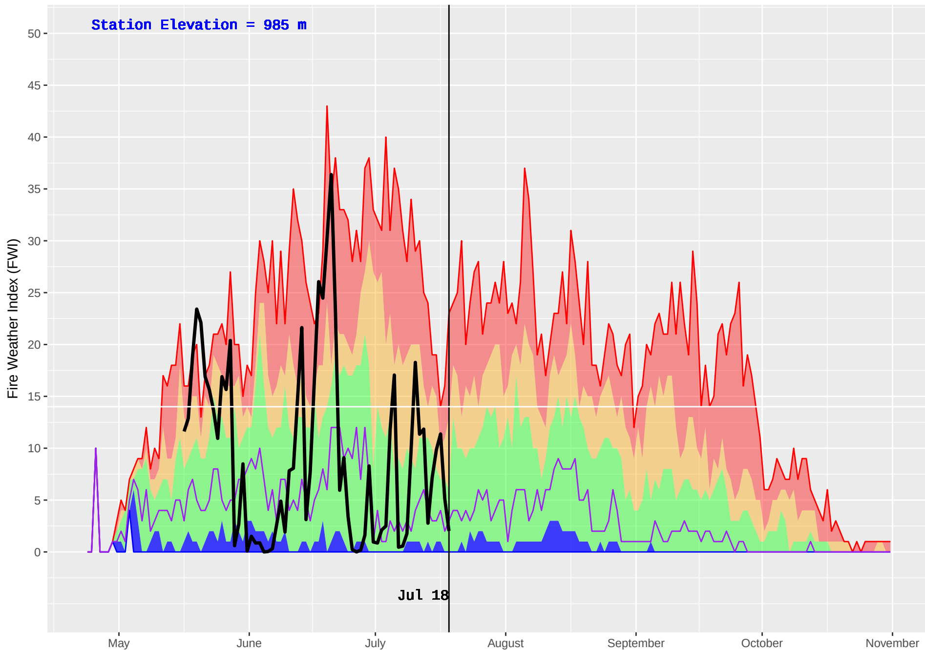
SIFTON (152) : Historical (1988–2016) and Current (2018) Daily Fire Weather Index (FWI)
