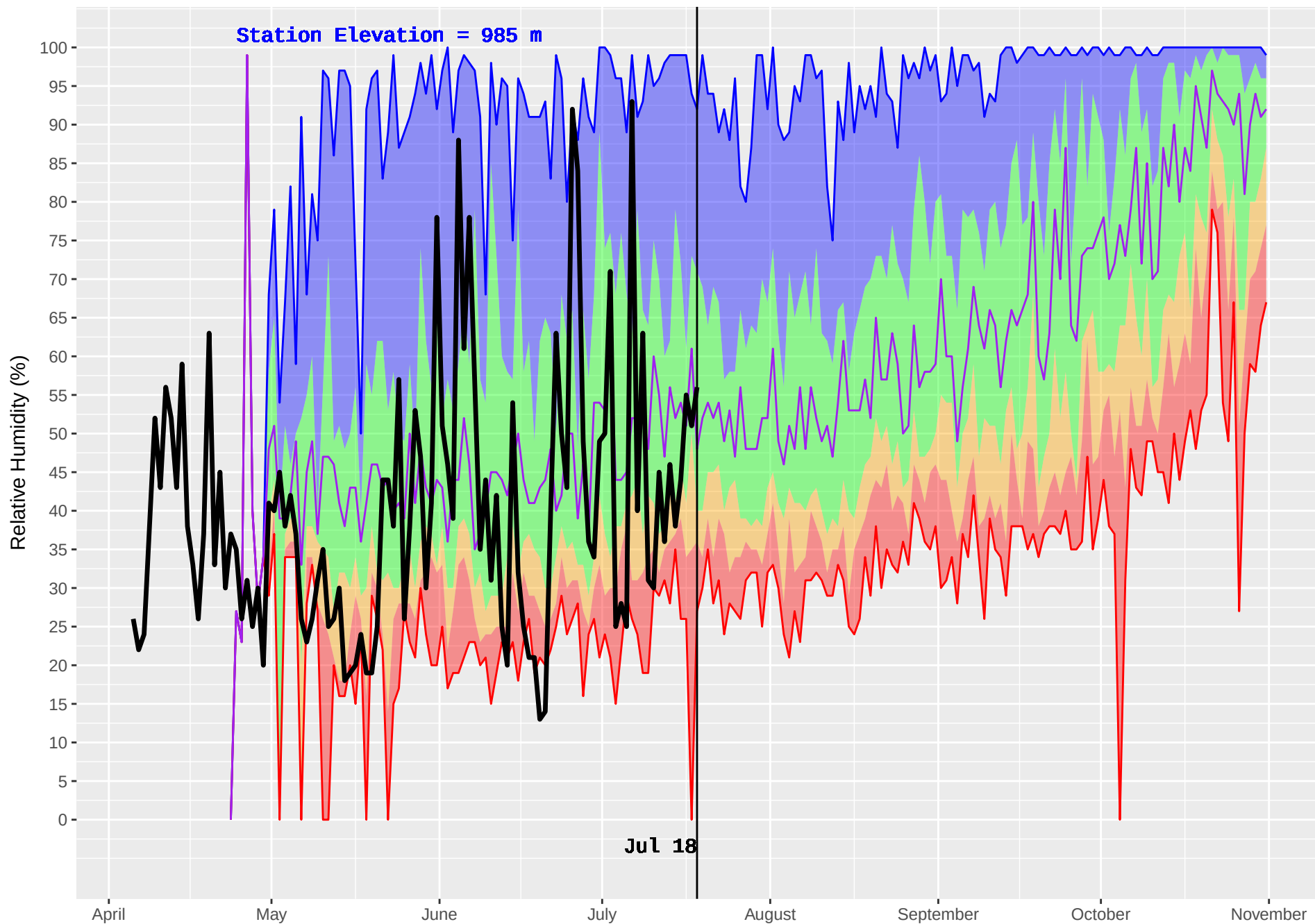
SIFTON (152) : Historical (1988–2016) and Current (2018) Daily Relative Humidity
