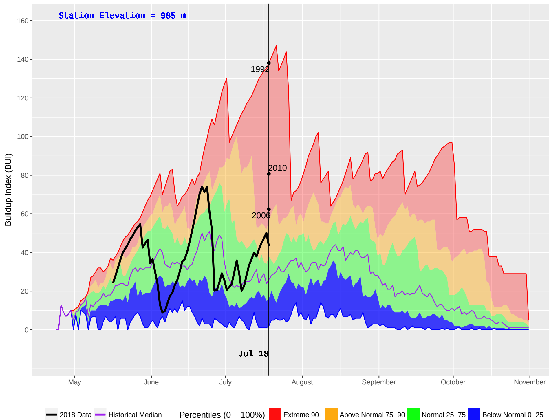
SIFTON (152) : Historical (1988–2016) and Current (2018) Daily Buildup Index (BUI)
