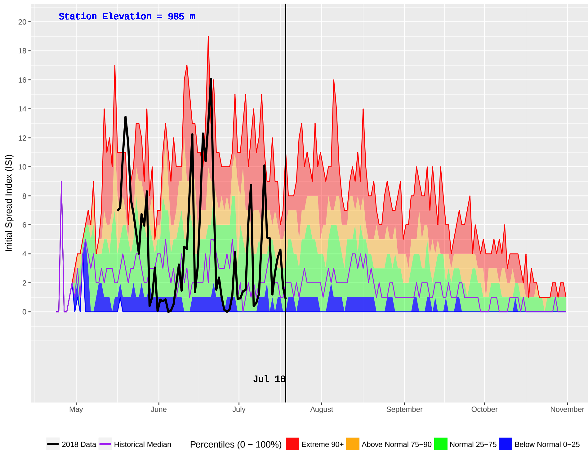
SIFTON (152) : Historical (1988–2016) and Current (2018) Daily Initial Spread Index (ISI)
