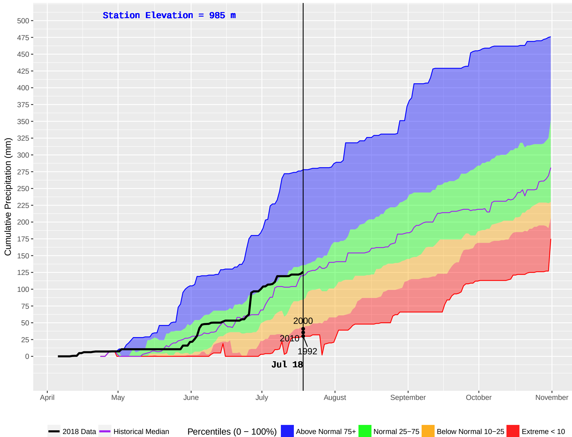
SIFTON (152) : Historical (1988–2016) and Current (2018) Daily Cumulative Precipitation
