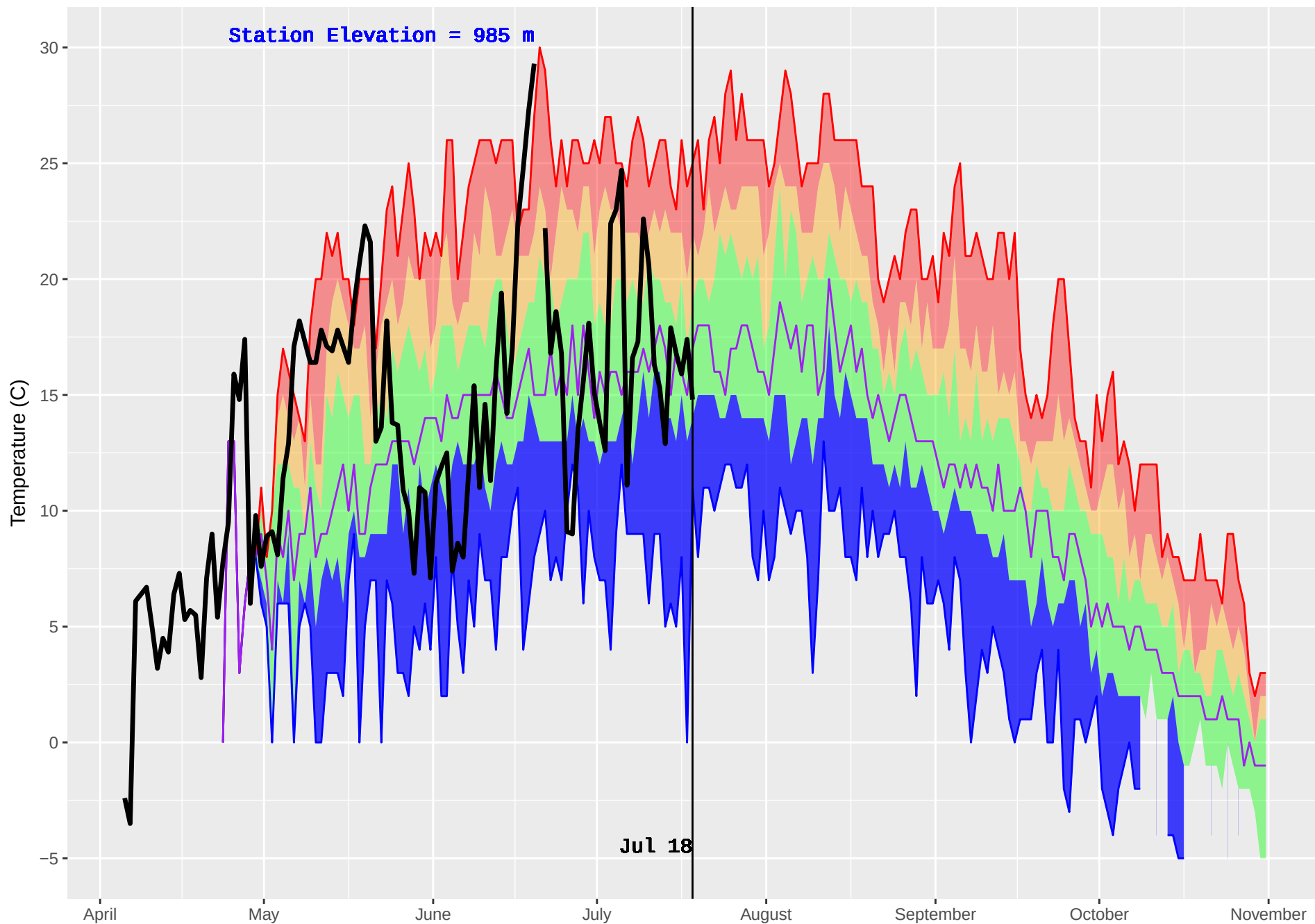
SIFTON (152) : Historical (1988–2016) and Current (2018) Daily Temperature
